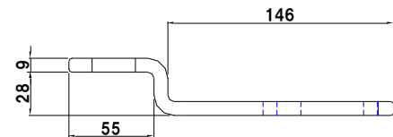
掛金9x65 3穴 28mm段
